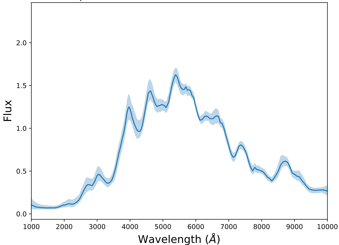
Spectrum 9 for transient SNIa at z=1.65
